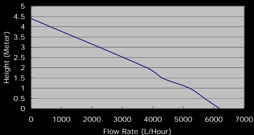
DC6000 Pump Performance
